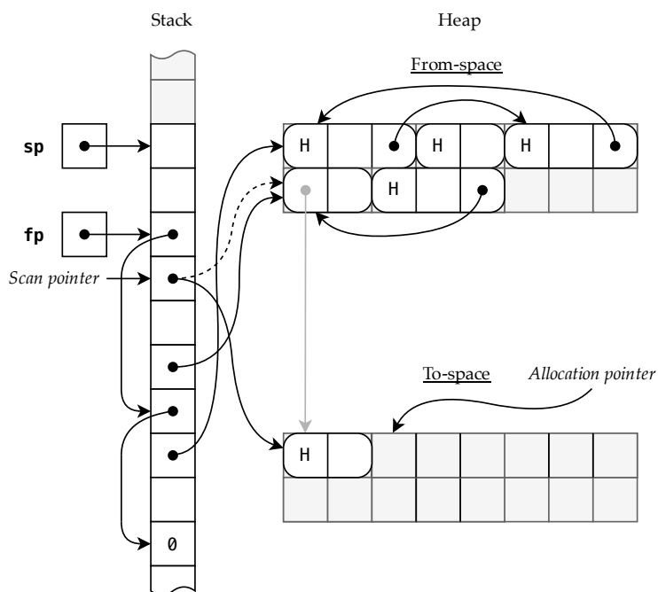
Figure 15.3: Scanning the stack: first pointer
