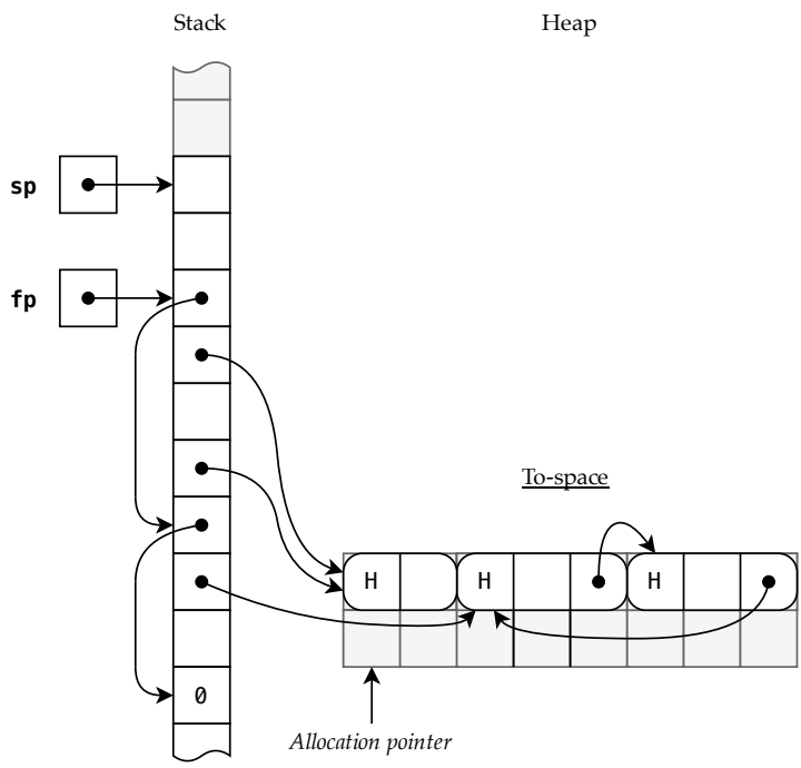
Figure 15.8: The state of our program after collection
