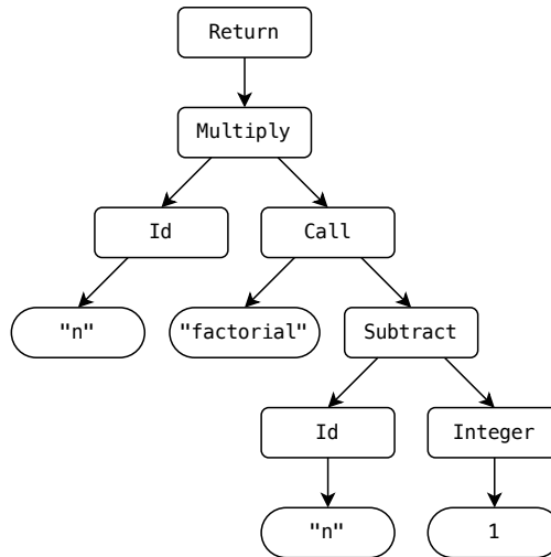
Figure 4.1: AST corresponding to return n * factorial(n - 1)
