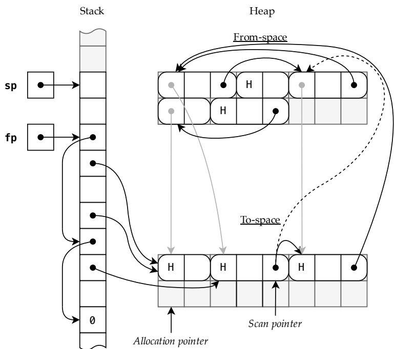
Figure 15.6: Scanning the to-space: first pointer
