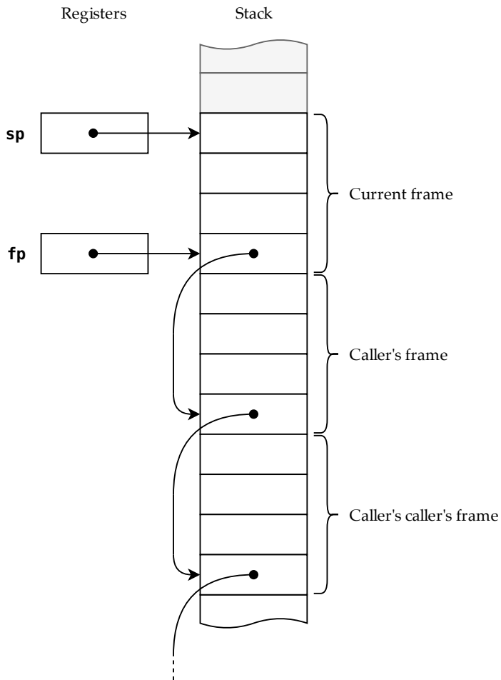
Figure 7.9: Example of a stack with several frames
