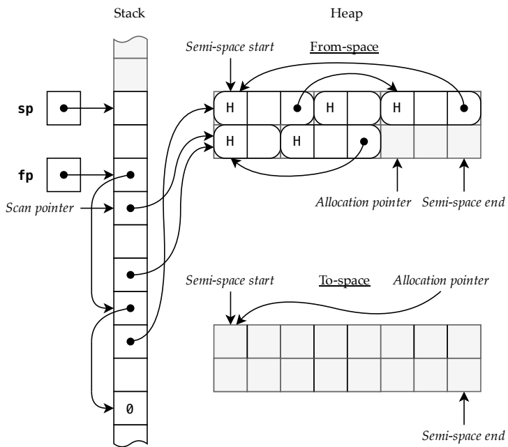
Figure 15.2: The two semi-spaces and their pointers
