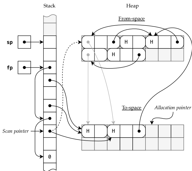
Figure 15.5: Scanning the stack: third pointer
