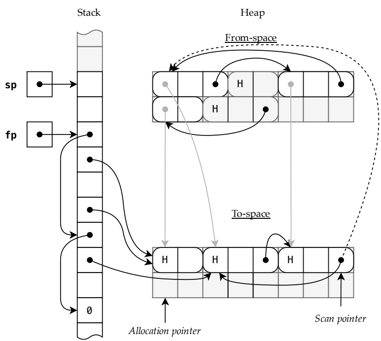
Figure 15.7: Scanning the to-space: second pointer
