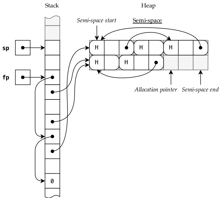
Figure 15.1: The state of our program: stack and heap
