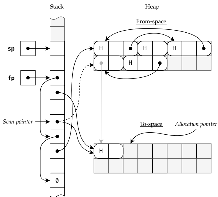
Figure 15.4: Scanning the stack: second pointer
