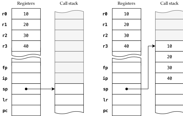
Figure 7.8: Call stack before and after executing: push {r0, r1, r2, r3}
