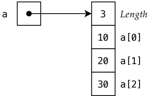
Figure 11.1: Word-diagram of a fixed-sized array layout
