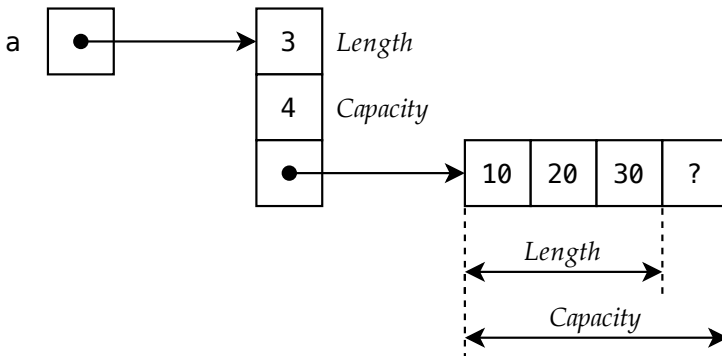
Figure 11.2: Word-diagram of a resizable array layout
